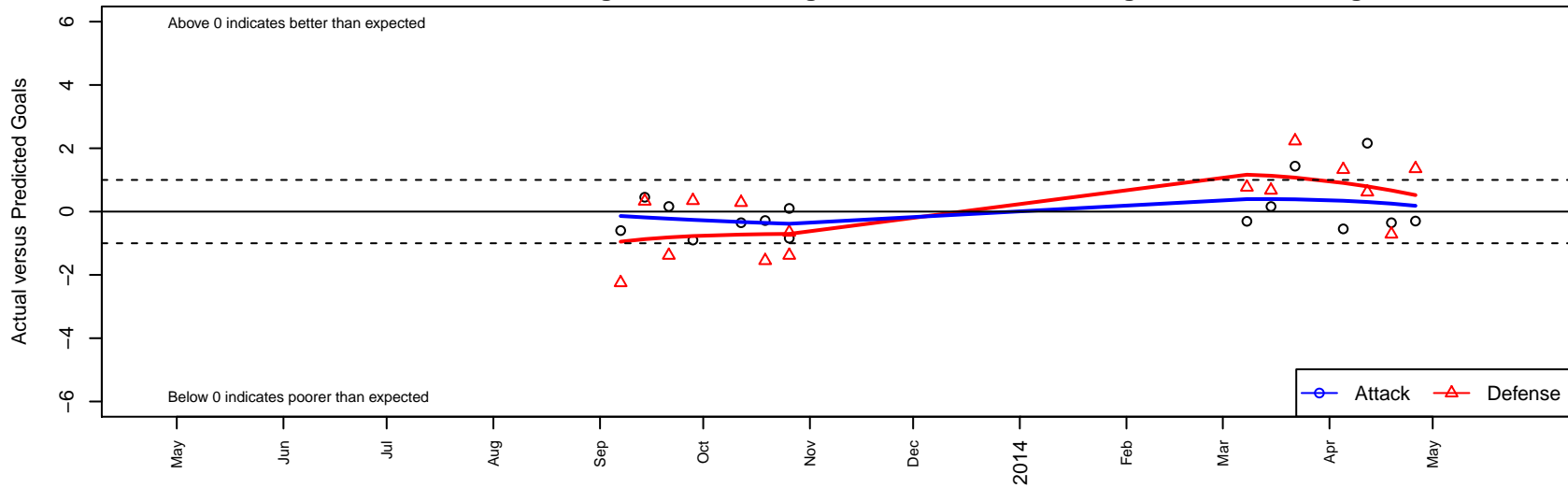
Mountain Home Sirens G99 Dots are actual minus expected GF (blue circles) and GA (red triangles). Blue line is smoothed change in attack strength. Red is smoothed change in defense strength.
